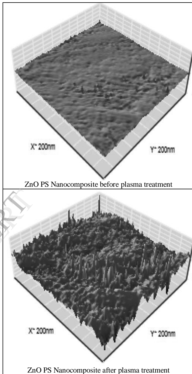
Fig. 4. AFM images of (a) 5 % ZnO doped PS membrane (b) 5% ZnO doped Plasma Treated Membrane.
